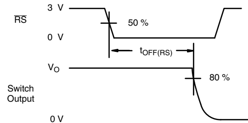
Figure 8. Reset Turn-Off Time t_{OFF(RS)}
